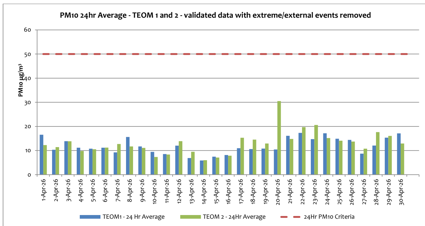
Figure 13: Site 1 and Site 2 PM 10 24-hour averaged measurements
