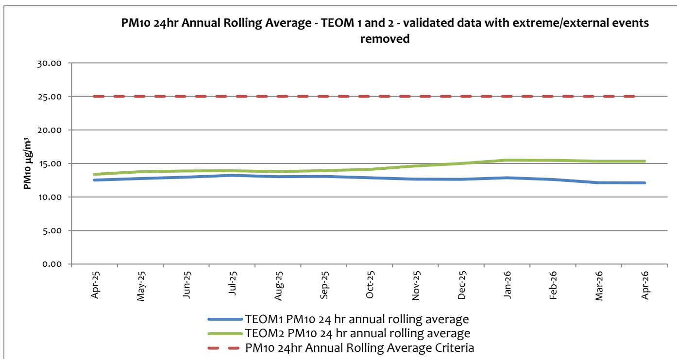
Figure 14: Site 1 & 2 - Annual rolling average PM 10 measurements 12-month overview
