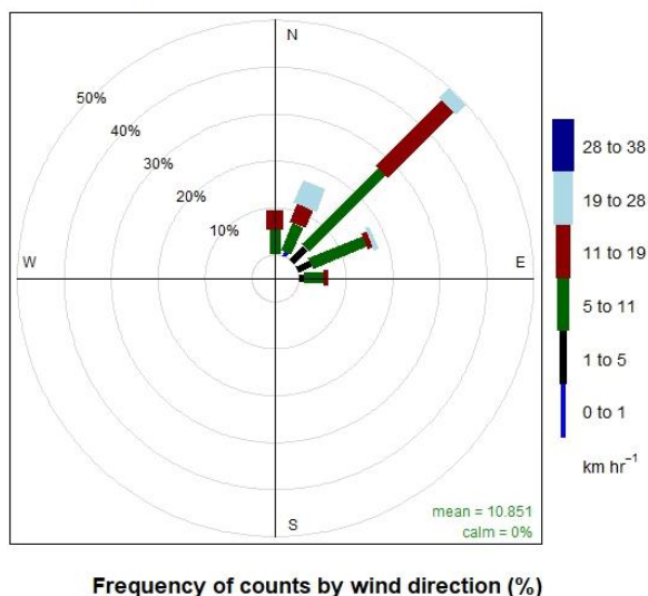
Broken Hill Operations Pty Ltd - Wind Rose 24 April 2026
