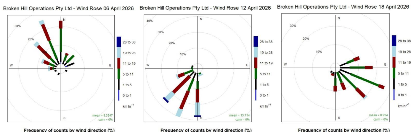
Figure 11: Wind roses for 06, 12 and 18 April, 2026
