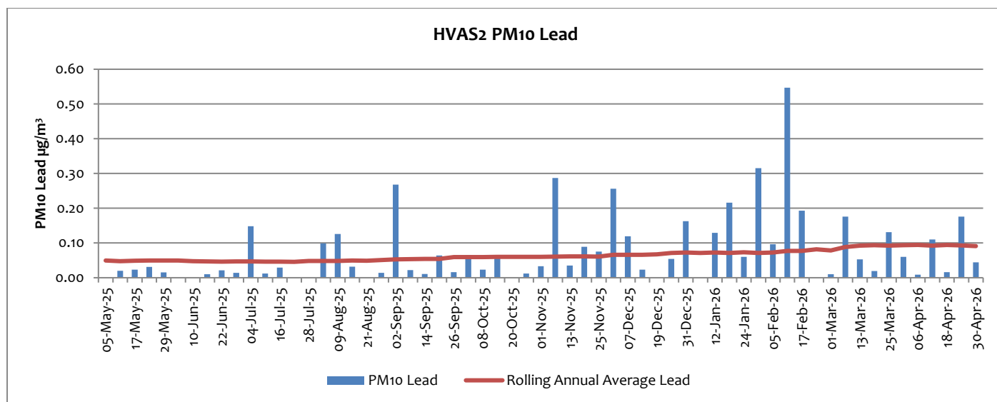
Figure 7: Lead in HVA502 PM 10 measurements 12-month overview
