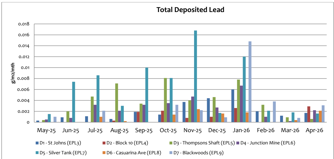
Figure 16: Lead deposited dust collected by 7 dust gauges - 12-month overview
