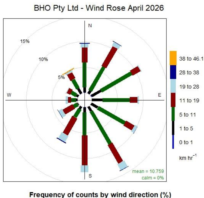
Figure 17: Wind rose for April 2026
